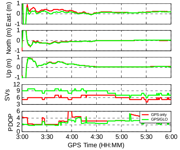
Fig. 11 Processing results at GOPE (Session 2)
