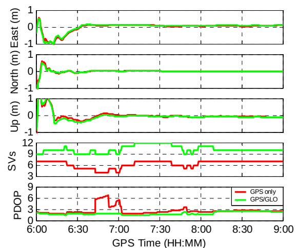
Fig. 8 Processing results at HERT (Session 3)
