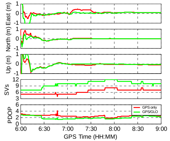
Fig. 12 Processing results at GOPE (Session 3)
