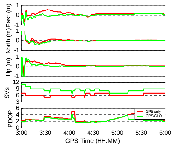
Fig. 7 Processing results at HERT (Session 2)
