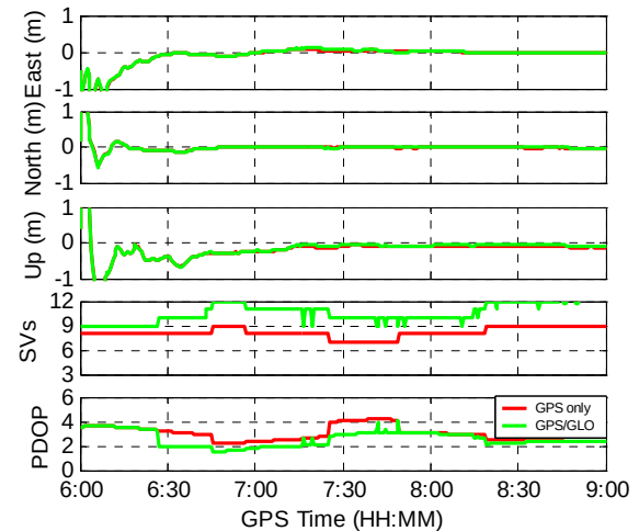
Fig. 16 Processing results at YARR (Session 3)
