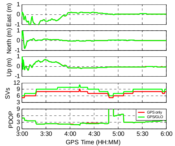
Fig. 15 Processing results at YARR (Session 2)
