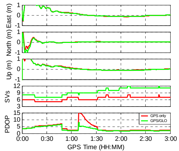
Fig. 6 Processing results at HERT (Session 1)
