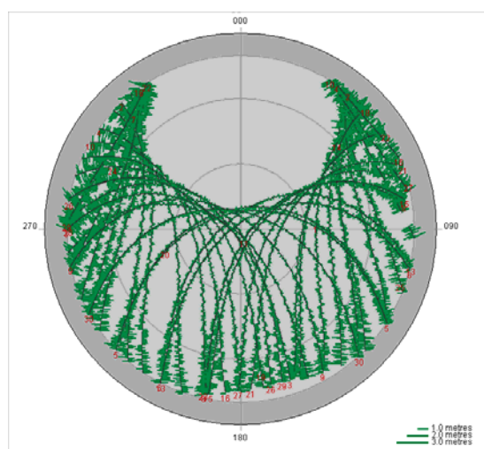
Fig. 4 MP1 sky plot for site FLDK
