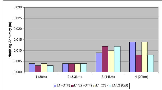
Fig. 9 Accuracy of Northing Component in Real Time (1 Sigma)
