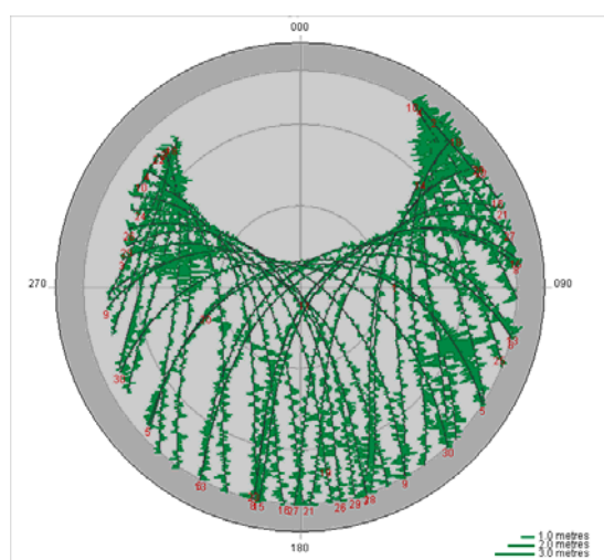
Fig. 6 MP1 sky plot for site RUTH
