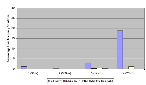
Fig. 8 Percentage of Solutions with Low Accuracy Position
