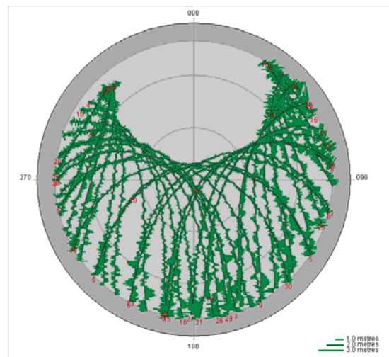
Fig. 3 MP1 sky plot for site BRON
