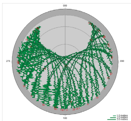
Fig. 5 MP1 sky plot for site KEW1
